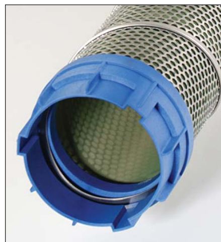
Open endcap with bayonet mount
