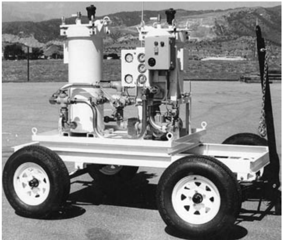
SDS20 Superdri Filter System mounted to off-road steerable trailer.
