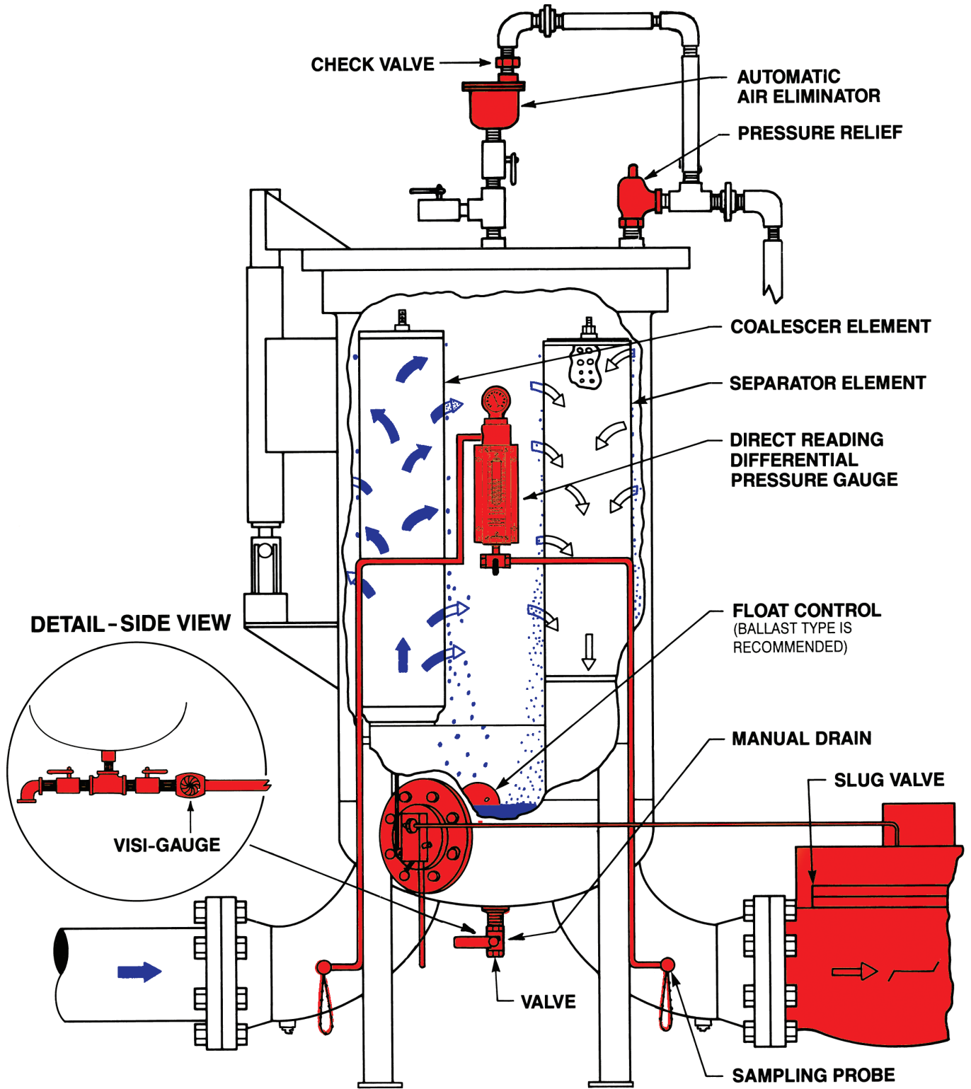
CUTAWAY—TYPICAL FILTER/SEPARATOR
