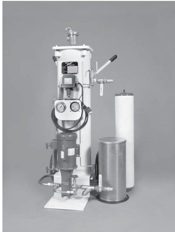
TOC5 shown with filter/coalescer cartridge and separator cartridge
