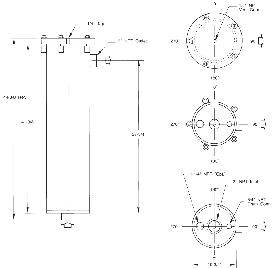
Standard VV-1033 Filter/Separator
